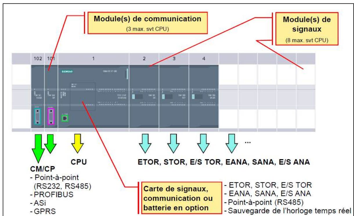
Figure 1.27 : Architecture de l'API S7-1200
